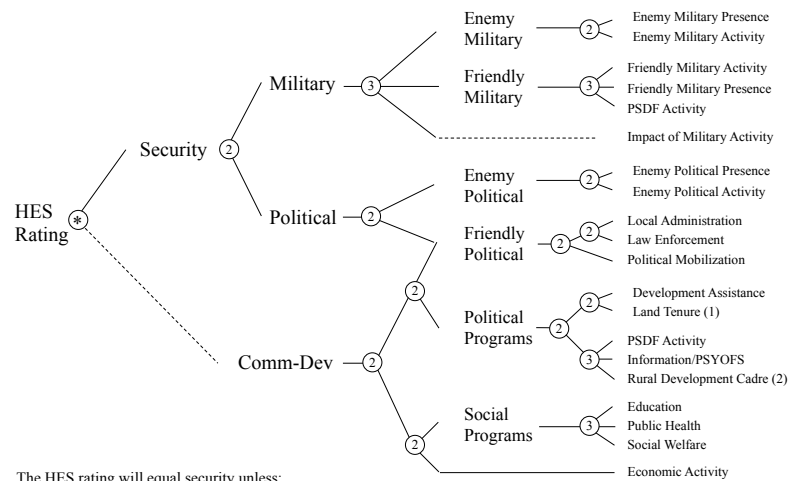
Figure II: Model Aggregation
