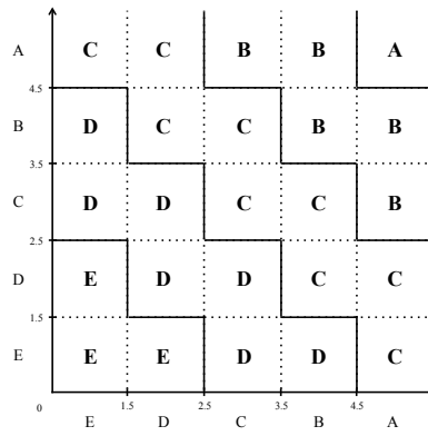
Figure I: Decision Logic (2-Way)
