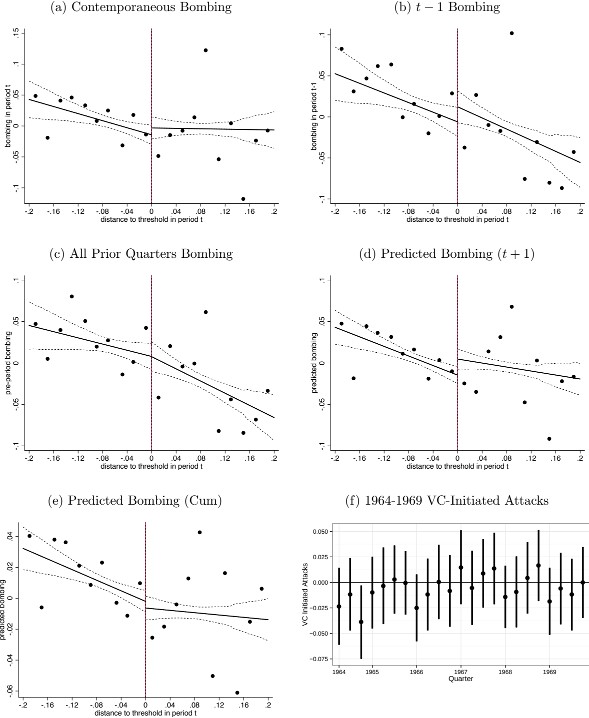
Figure IV: Placebos
