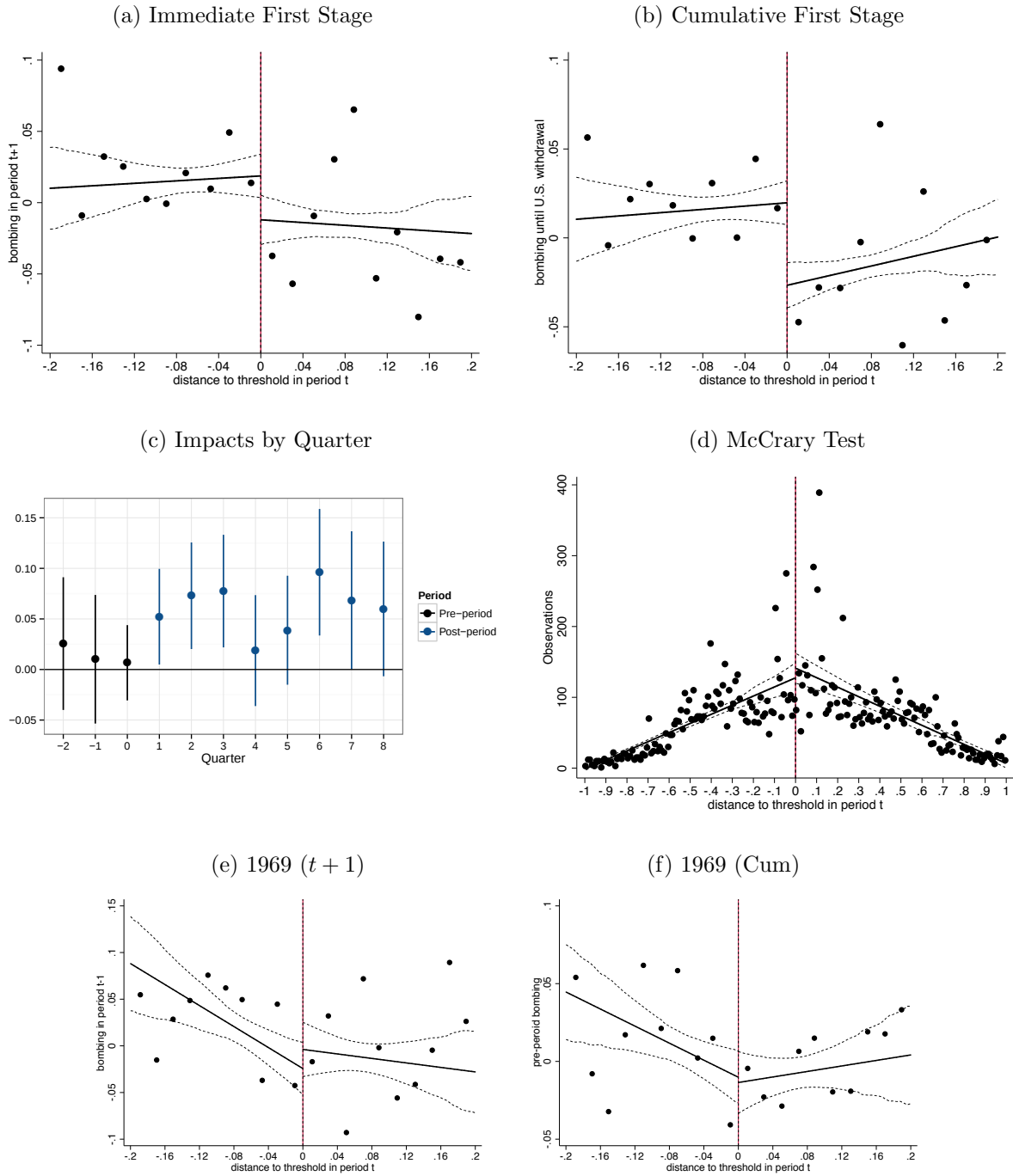
Figure III: First Stage
